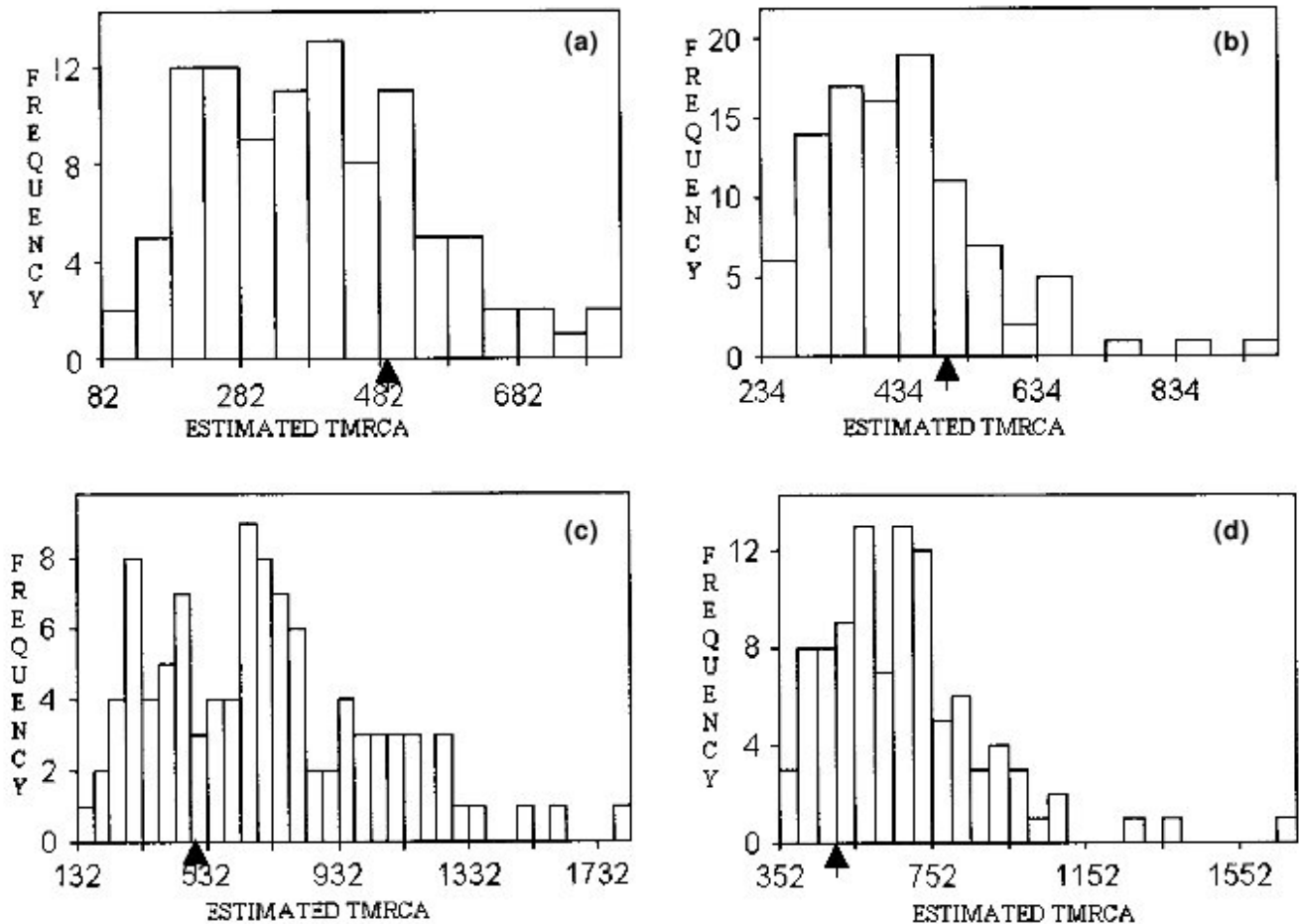
Figure 3. Frequency distributions of TMRCA estimated by two methods on simulated DNA sequence data, with simulation parameters L = 400 nucleotides, \mu = 5 \times 10^{-5} per site per generation and g = 500 generations (marked with an arrow on the X-axis), comprising 100 replications of each data set. (a) \alpha = 0 , Templeton's estimation method; (b) \alpha = 0.005 , Templeton's estimation method; (c) \alpha = 0 , MJN estimation method; (d) \alpha = 0.005 , MJN estimation method.
