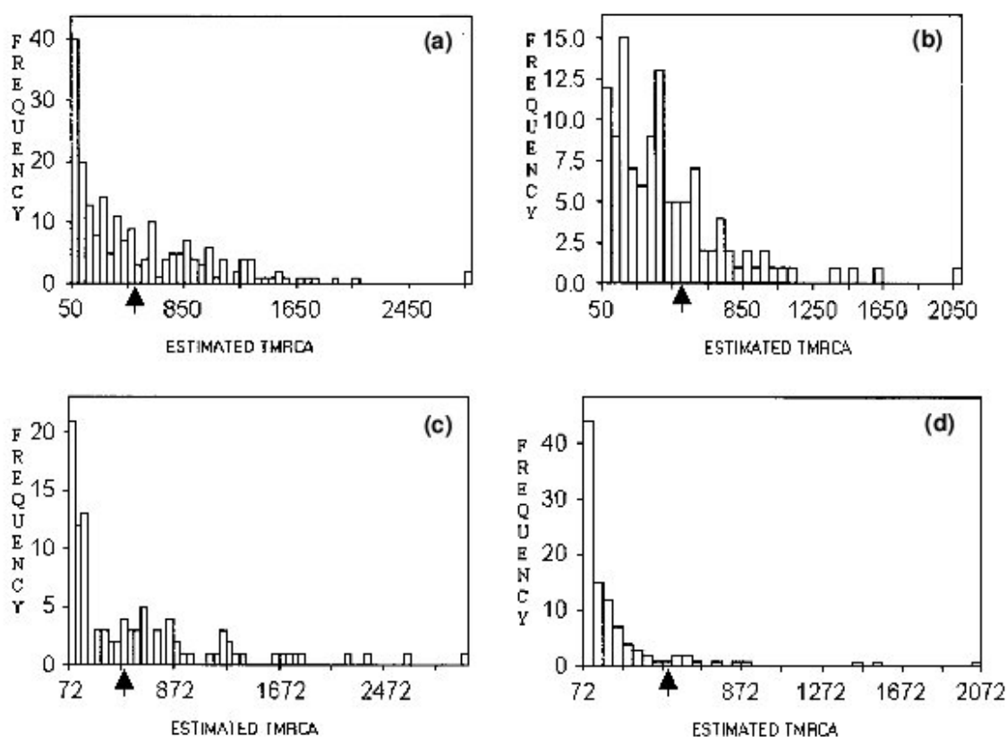
Figure 2. Frequency distributions of TMRCA estimated by two methods on simulated DNA sequence data, with simulation parameters L = 200 nucleotides, \mu = 10^{-5} per site per generation and g = 500 generations (marked with an arrow on the X-axis), comprising 100 replications of each data set. (a) \alpha = 0 , Templeton's estimation method; (b) \alpha = 0.005 , Templeton's estimation method; (c) \alpha = 0 , MJN estimation method; (d) \alpha = 0.005 , MJN estimation method.
