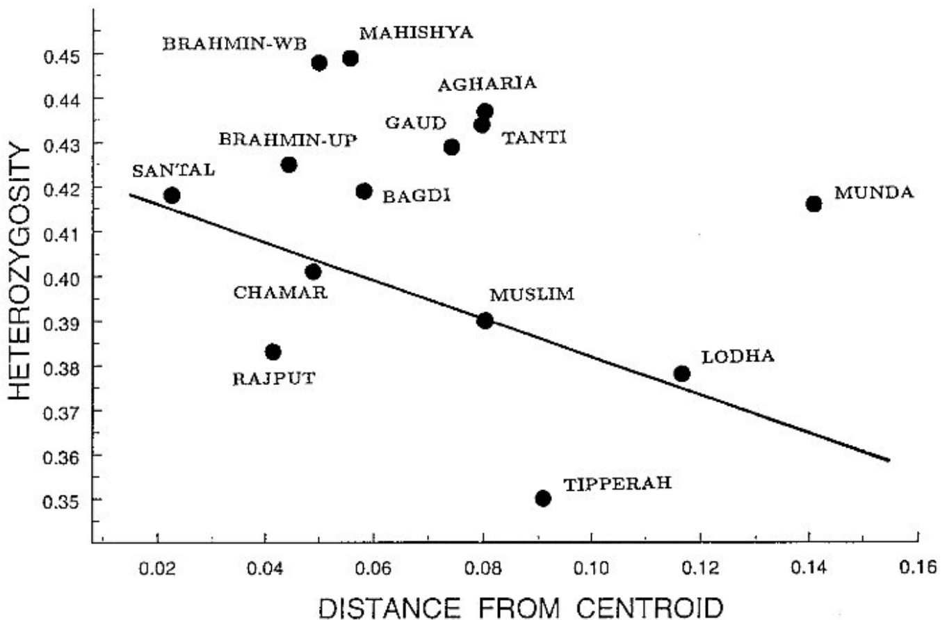
Figure 4 Plot of average heterozygosity vs distance from allele frequency centroid of 14 Indian ethnic populations based on allele frequency data of eight loci.
