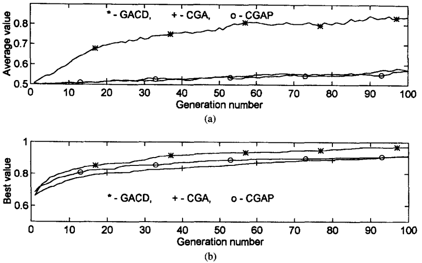
Fig. 7. (a) Variation of average value of objective function with generations for function 6 (Sine square function). (b) Variation of best value of objective function with generations for function 6 (Sine square function).
