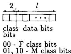
Fig. 2. Structure of a chromosome in GACD.
