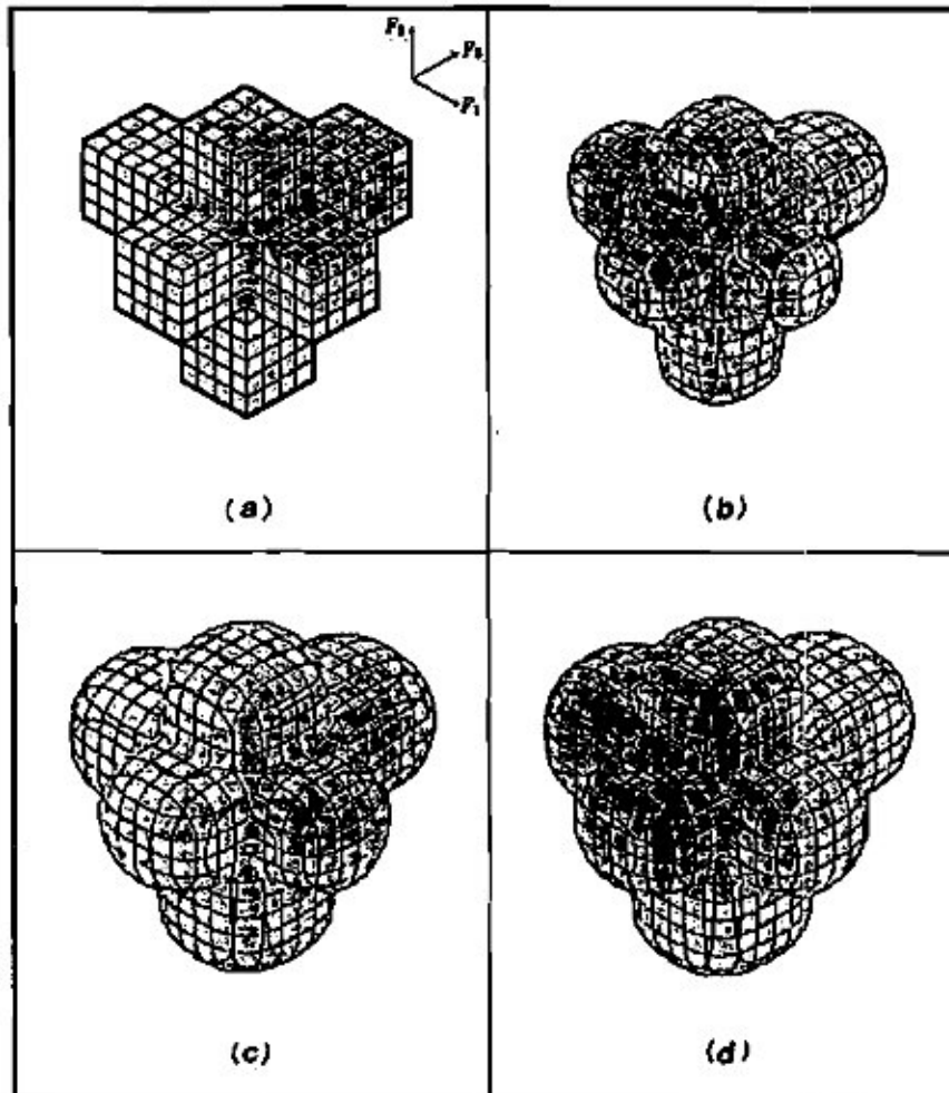
FIGURE 6 (a) A pattern class; (b)–(d) corresponding estimated versions with \theta \cong 0.5 , \theta \cong 0.25 , \theta > 0 respectively.
