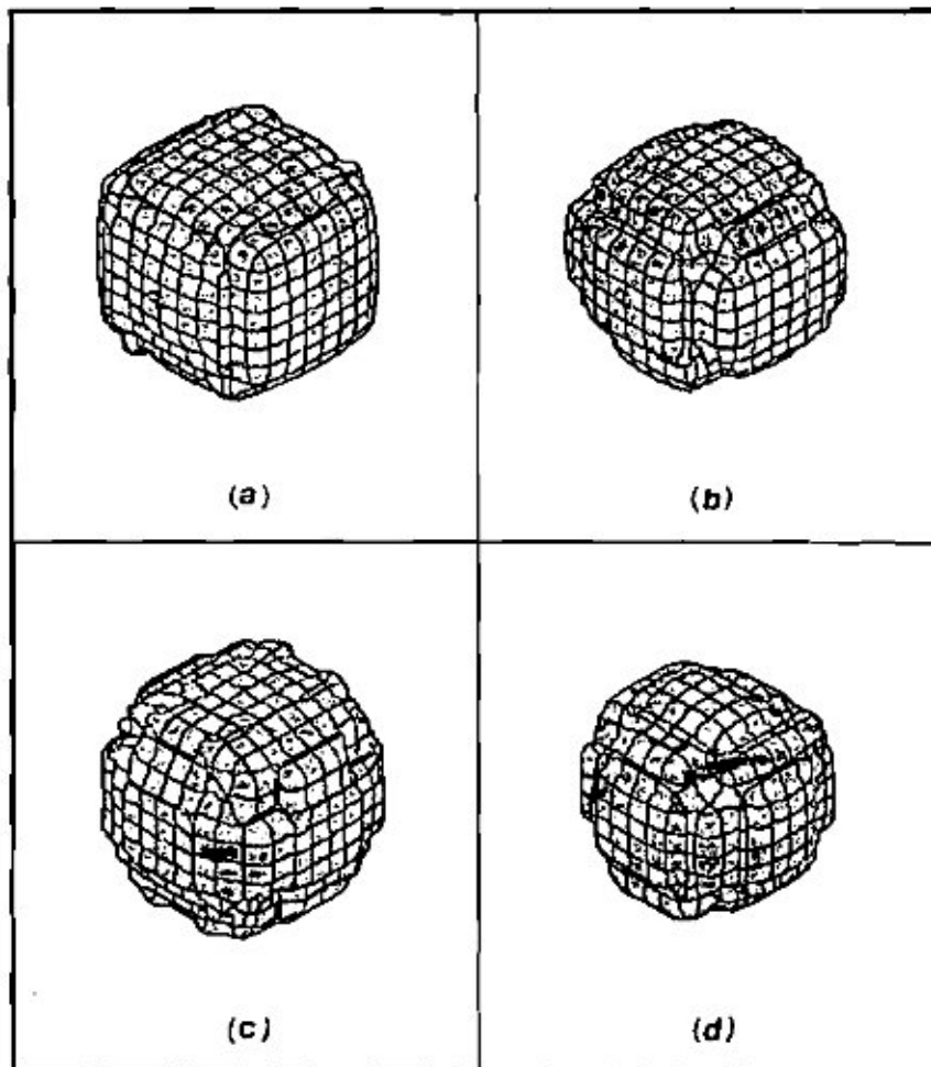
FIGURE 10 (a)–(d) Estimated versions of the class in Fig. 9 with \theta \cong 0.5 based on 150, 300, 500 and 1200 samples respectively.
