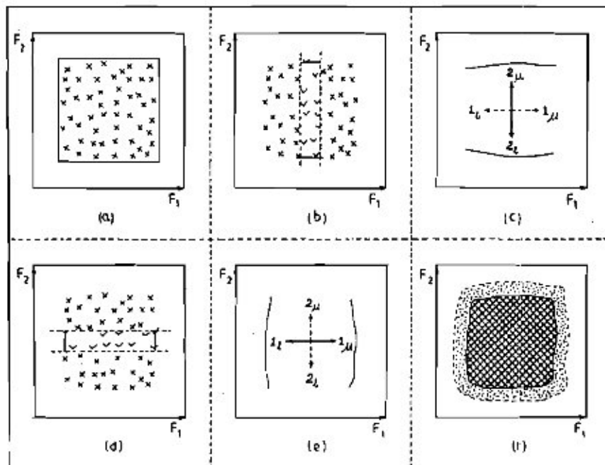
FIGURE 2 Illustrating the concept of boundary in R^2 .
