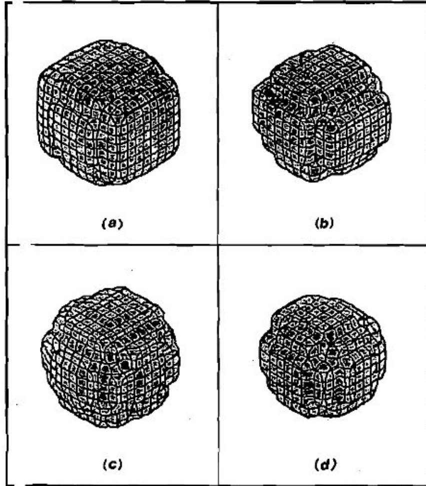
FIGURE 11 (a)–(d) Estimated versions of the class in Fig. 9 with \theta \geq 0.25 based on 150, 300, 500 and 200 samples respectively.
