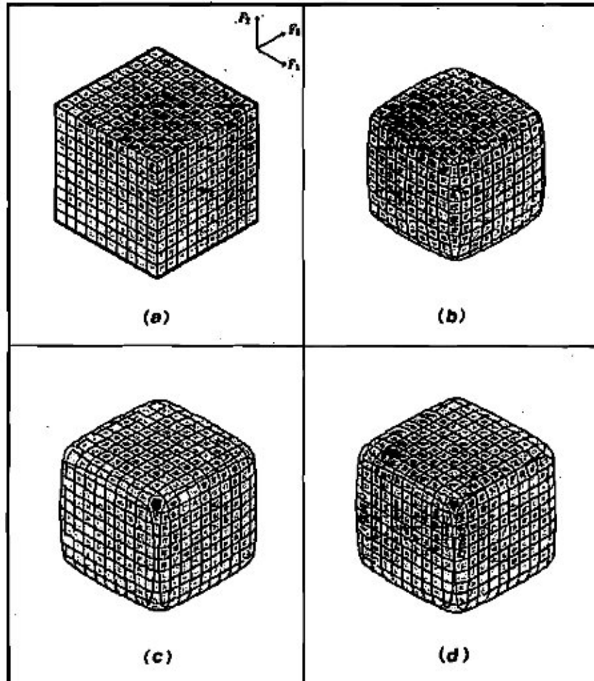
FIGURE 5 (a) A pattern class; (b)–(d) corresponding estimated versions with \theta \approx 0.5 , \theta \approx 0.25 , \theta > 0 respectively.
