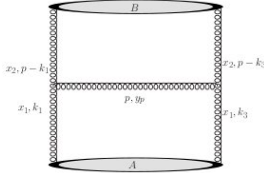
FIG. 3: Single-particle production from k_{\perp} -factorization at leading order. The blobs denote the unintegrated gluon distribution of the projectile A or target B , respectively.
