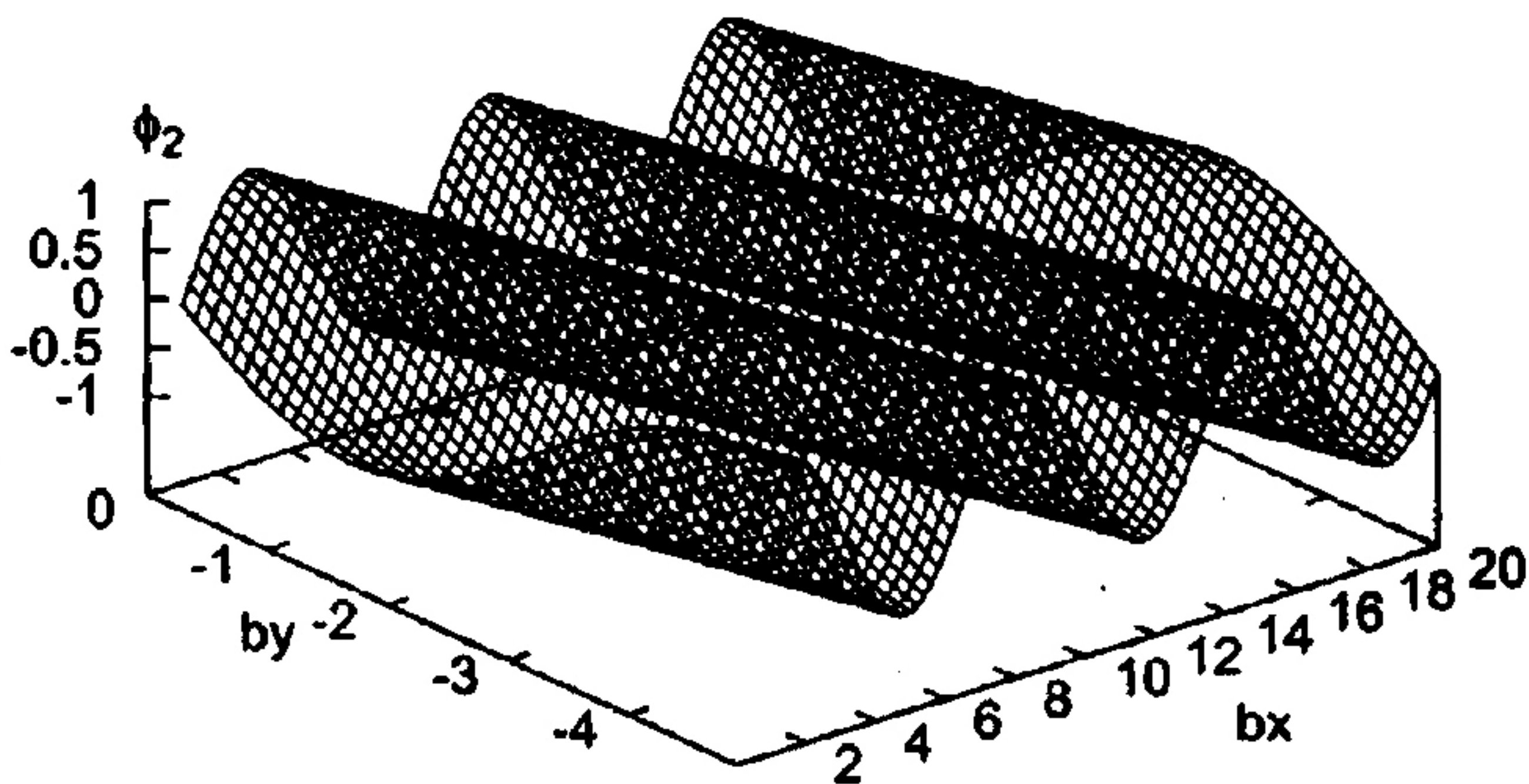
Fig. 1. Waves reflected from the inertial surface
