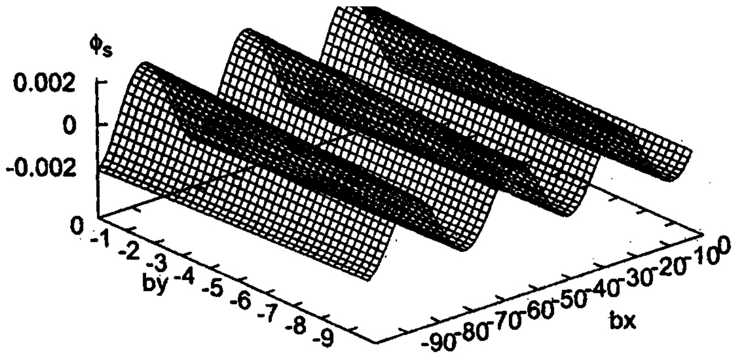
Fig. 5. Waves under the free surface in \pi - \theta_c < \theta < \pi
