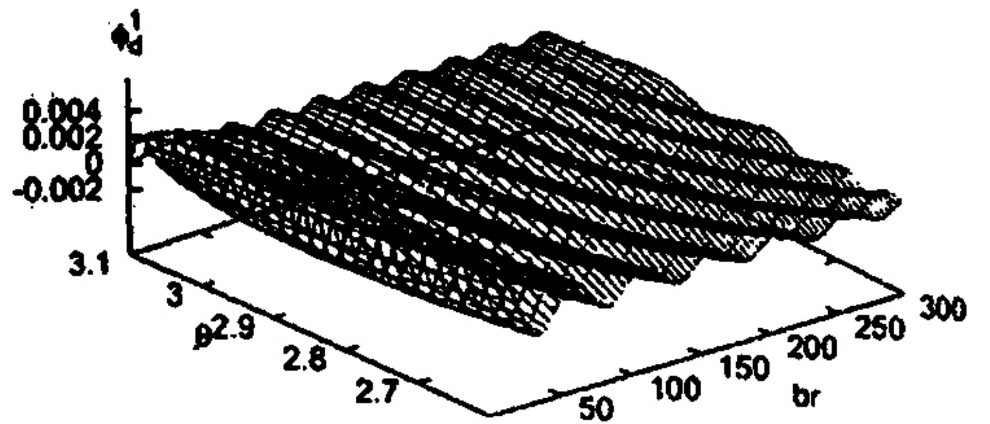
Fig. 3. Waves due to diffraction in \pi - \theta_c < \theta < \pi
