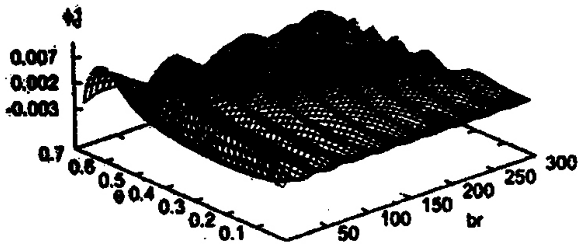
Fig. 2. Waves due to diffraction in 0 < \theta < \theta_c
