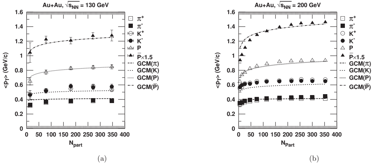
Fig. 7. Nature of average transverse momenta ( \langle p_T \rangle ) for various secondaries produced in AuAu collisions at two different energies as a function of N_{part} . The data-type points are the extracted-results obtained by RHIC experimental groups[1]. The GCM-based results are shown by various dashed and dotted curves.
