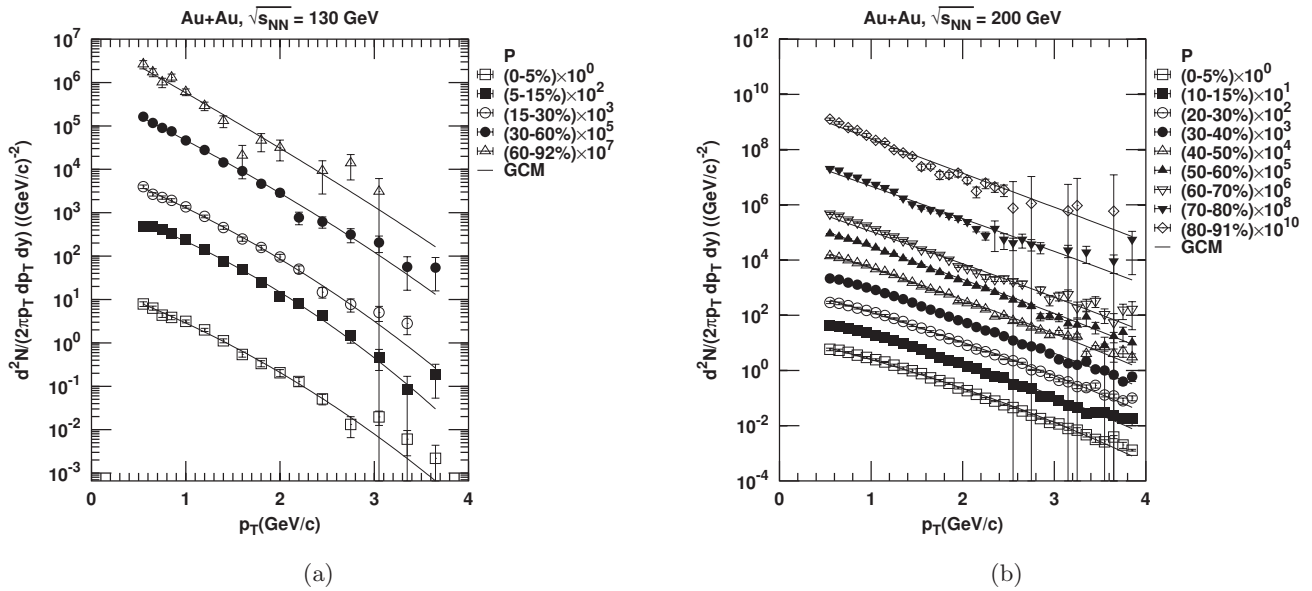
Fig. 4. Plots of invariant spectra for production of secondary protons in AuAu collisions at two different RHIC-energies at different centralities. The various experimental data points at \sqrt{s_{NN}} = 130 GeV are taken from Ref.[18] while those for \sqrt{s_{NN}} = 200 GeV are from Ref.[1]. The GCM-based fits are depicted by the solid curves.
