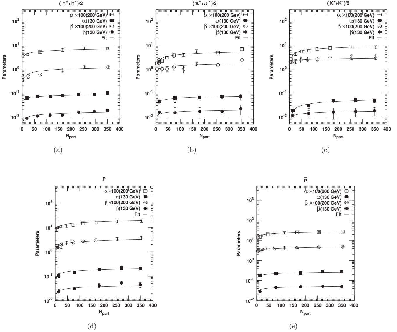
Fig. 6. Plots of \alpha [in (c/GeV)] and \beta [in (c/GeV) 2 ] as a function of number of participant nucleons, N_{part} . The different data-type points for various secondaries are taken from Table 2 - Table 11. Various solid curves are drawn on the basis of eqn.(9) and denoted as 'Fit' in the figures.
