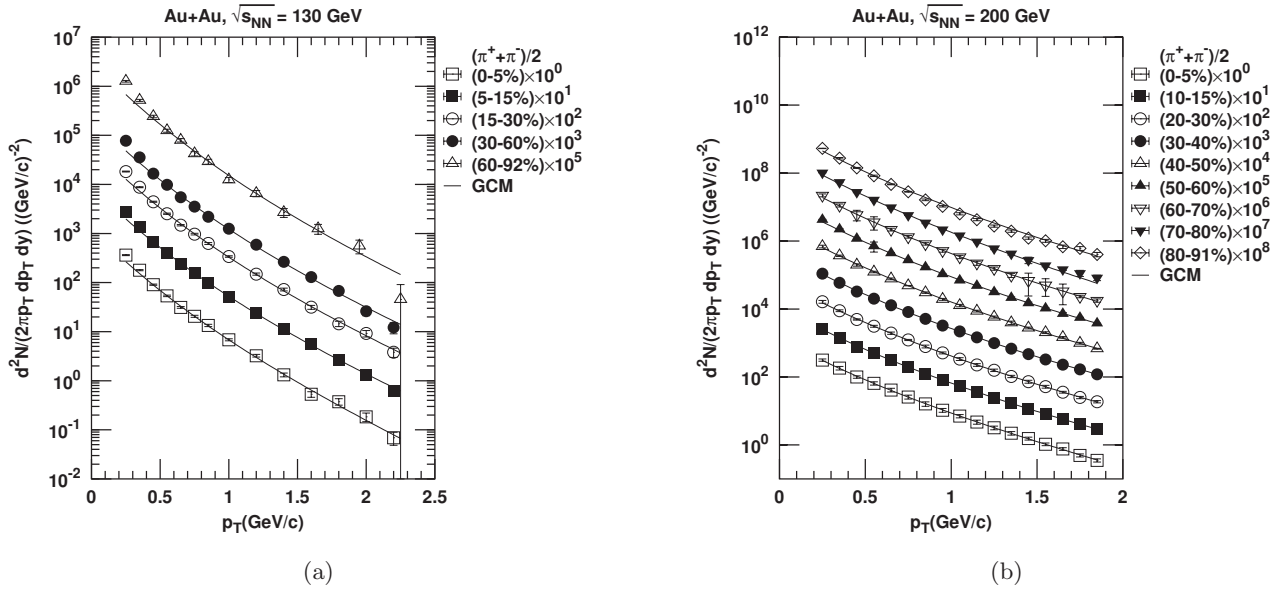
Fig. 2. Nature of invariant spectra of secondary charged pions produced in AuAu collisions at two different RHIC-energies at different centralities as a function of p_T . The experimental data points at \sqrt{s_{NN}} = 130 GeV are taken from Ref.[18] while those for \sqrt{s_{NN}} = 200 GeV are from Ref.[1]. The solid curves are drawn on the basis of eqn.(6).
