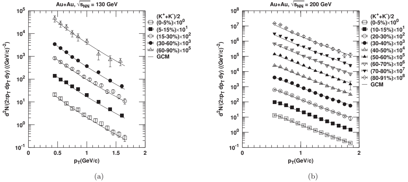
Fig. 3. Transverse momentum spectra for production of secondary charged kaons in AuAu collisions at two different RHIC-energies at different centralities. The various experimental data points at \sqrt{s_{NN}} = 130 GeV are taken from Ref.[18] while those for \sqrt{s_{NN}} = 200 GeV are from Ref.[1]. The present model(GCM)-based fits are depicted by the solid curvilinear lines.
