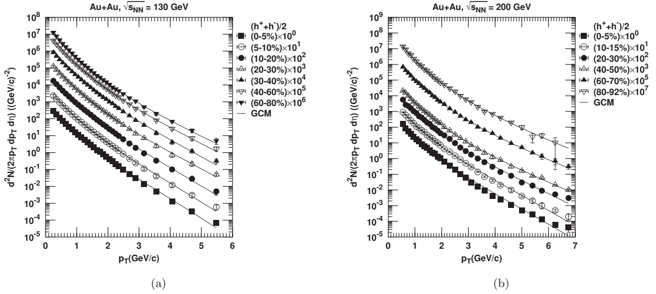
Fig. 1. Plots of invariant spectra of secondary charged hadrons produced in AuAu collisions at two different RHIC-energies for various centrality-bins. The experimental data points are taken from Ref.[17] for \sqrt{s_{NN}} = 130 GeV and from Ref.[3] for \sqrt{s_{NN}} = 200 GeV. The solid curves provide the GCM-based fits.
