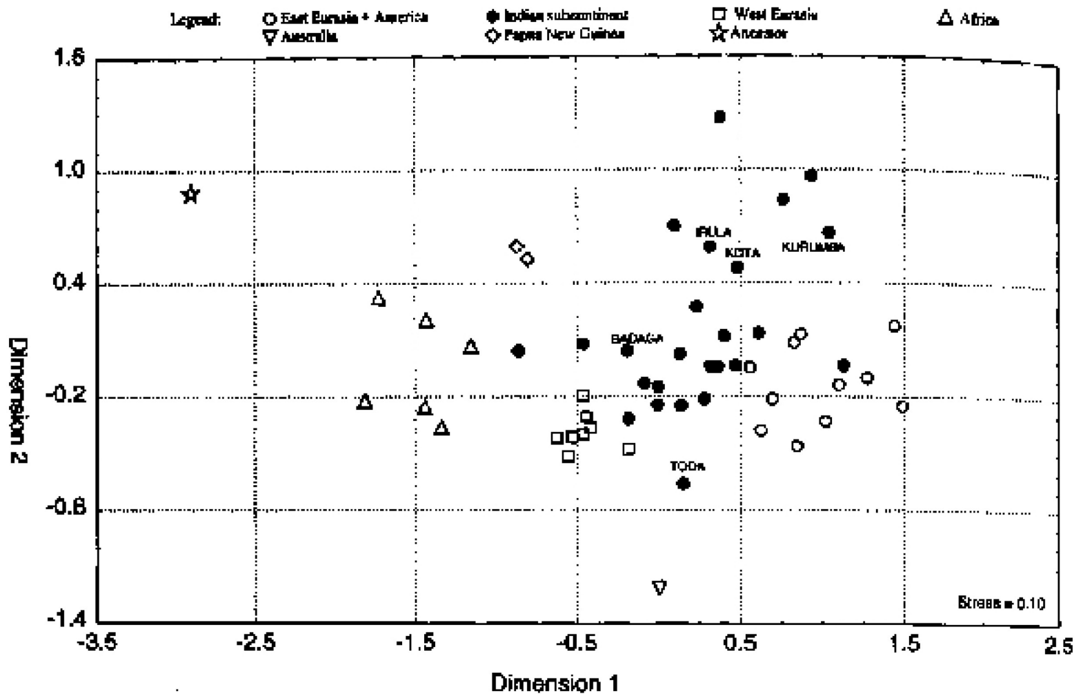
Figure 3 Multidimensional scaling plot depicting the genetic relationships of 54 world populations, using five Alu insertion loci ( AluACE , AluFXIIB , AluAPO , AluPV92 , AluPLAT ). A hypothetical ancestral population is shown, in which the frequency of the Alu element at each locus is set to 0.
