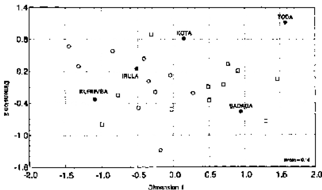
Figure 2 Multidimensional scaling plot depicting the genetic relationships of 26 Indian populations based on seven insertion/deletion loci (mtNUC, Alu PV92, Alu FXIIIIB, Alu APC, Alu ACE, Alu Plat and CD4del). Filled circles represent Nilgiri Hills' tribal populations; open circles represent other tribal groups; open squares represent non-tribal groups.
