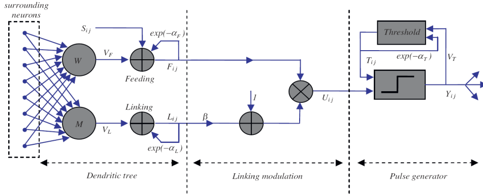
Fig. 1 Structure of PCNN.
