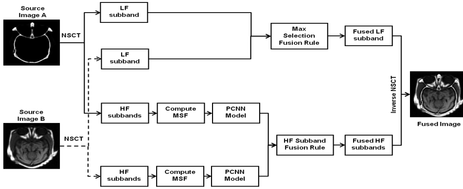
Fig. 2 Block diagram of the proposed MIF method.
