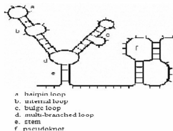
Fig. 1. Different types of secondary substructures in RNA
