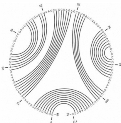
Fig. 3. A circular representation of RNA secondary structure [6].
