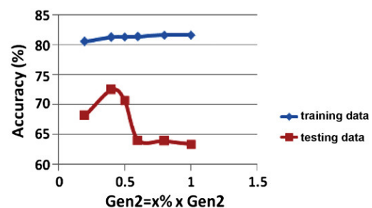
(b) Classification accuracy of Metabolic Syndrome dataset
