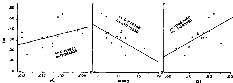
Figure 2. Bivariate scatters and fitted regression line between I_m and \alpha , MMD, and DI, respectively.
