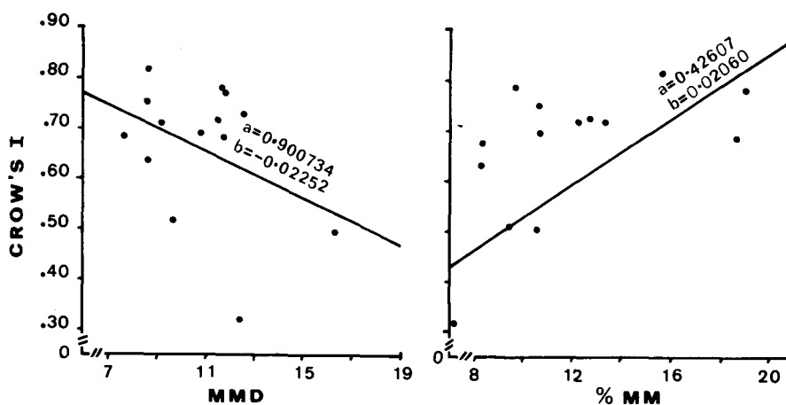
Figure 3. Bivariate scatters and fitted regression line between I_t and MMD, and MM, respectively.
