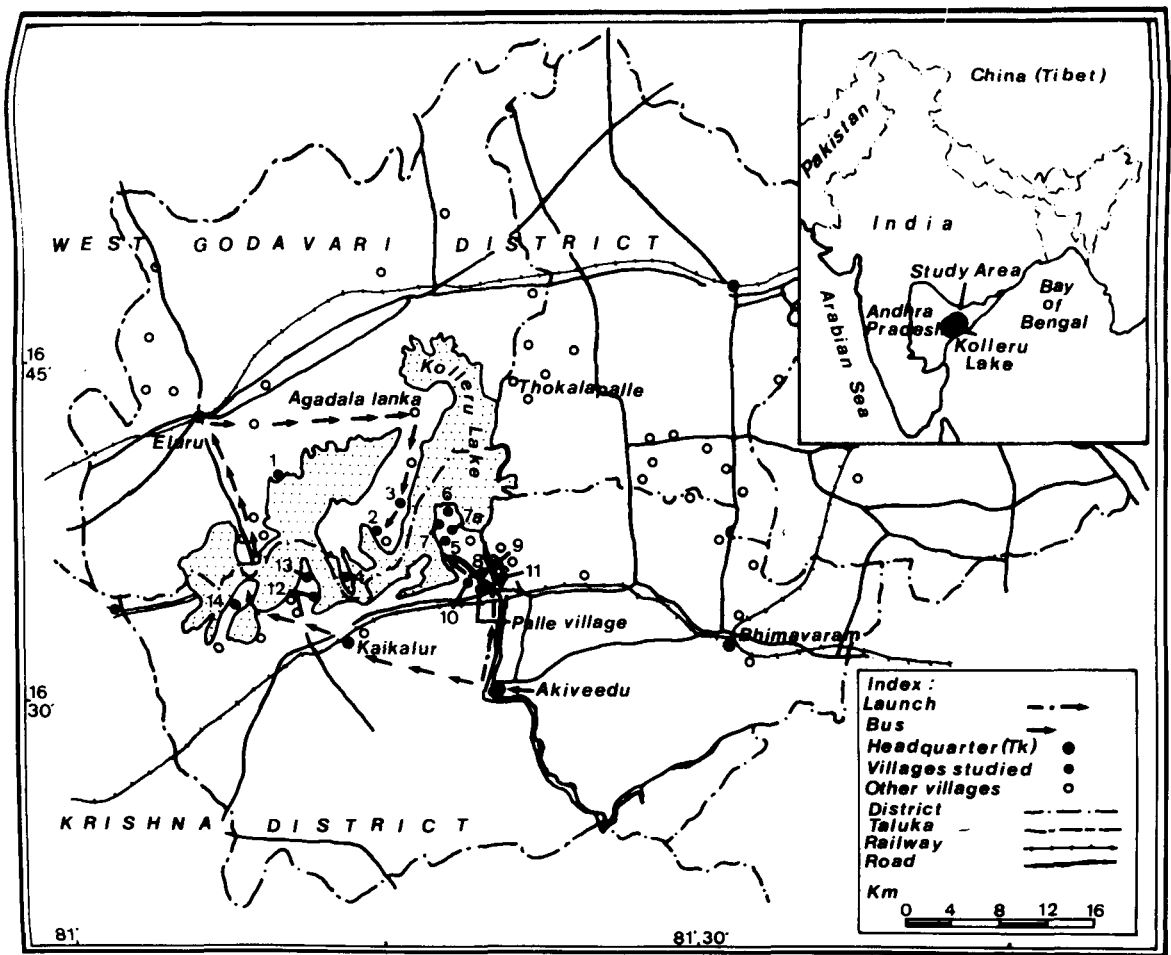
Figure 1. Map showing the geographical location of villages in the region of Kolleru Lake.
