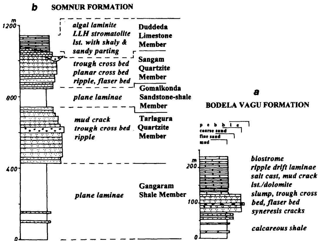
Fig. 2. Generalised Lithologs of the Bodela Vagu Formation (a) and the Somnur Formation (b).
