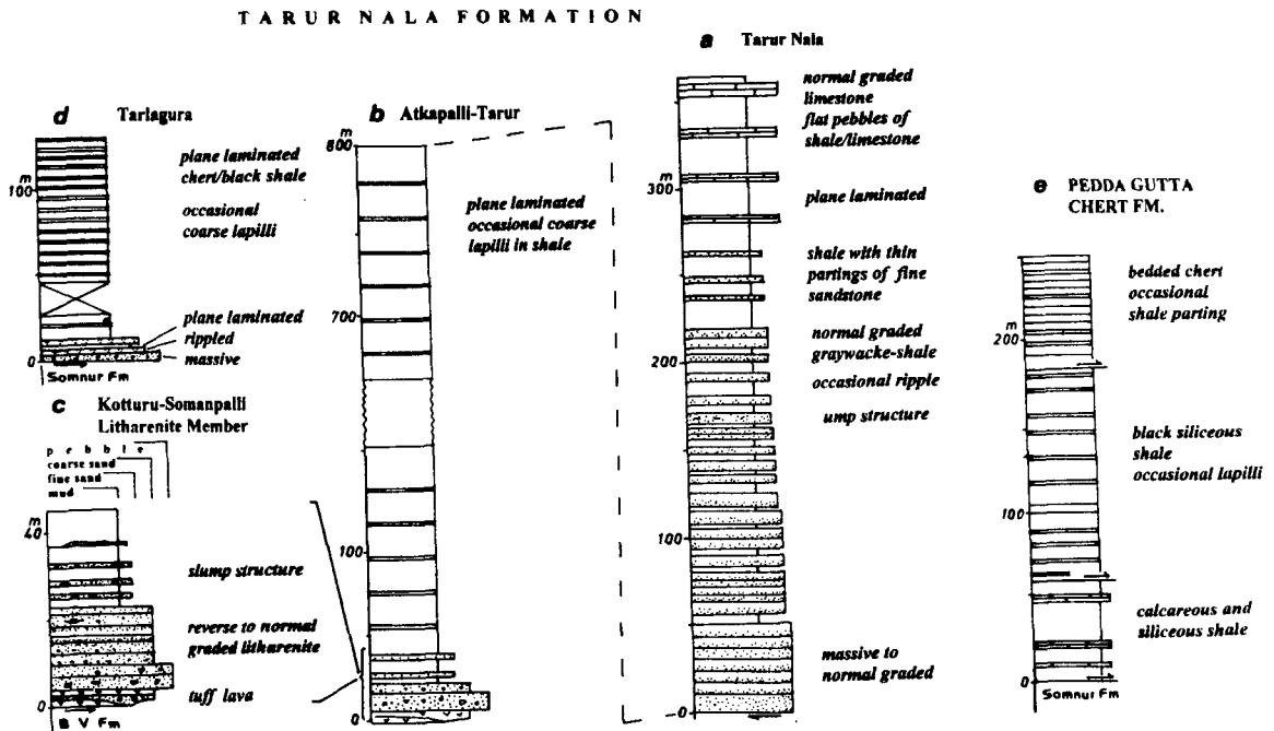
Fig. 3. Lithologs of the Tarur Nala Formation from Tarur Nala and other sections, and generalised log for the Pedda Gutta Chert Formation. Arrows indicate fault contacts.
