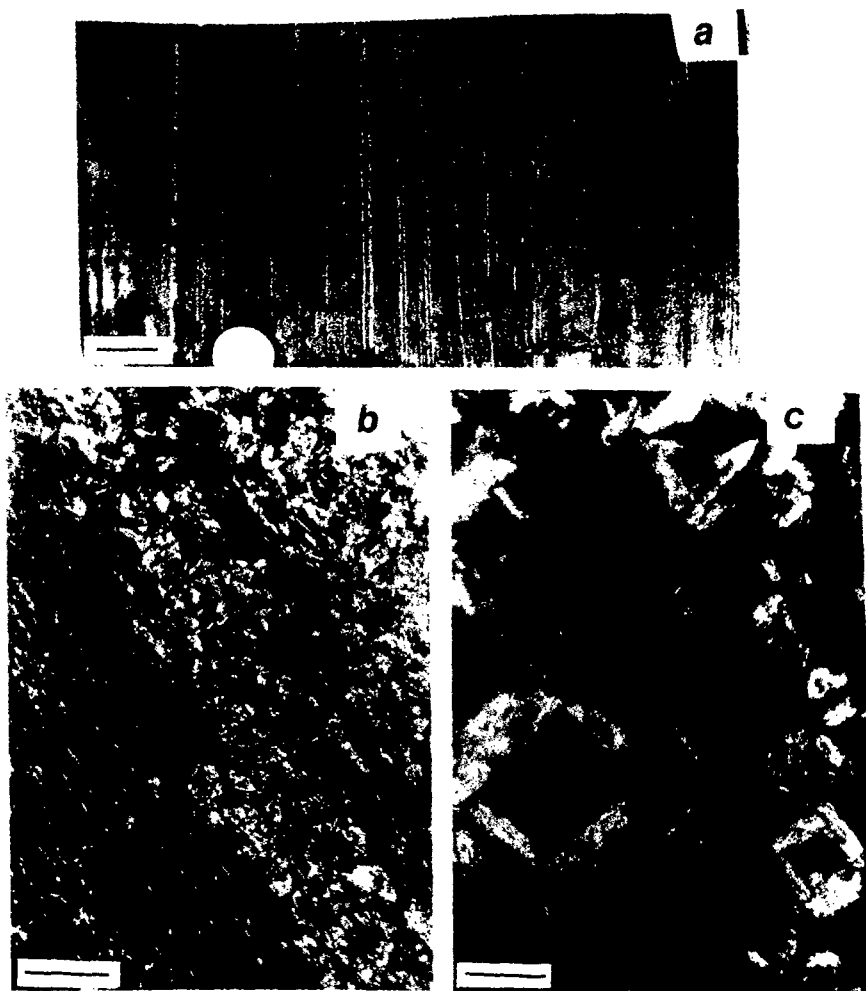
Fig. 4. Ash beds, Indravati River bed off Kotturu-Somanpalli. (a) Field photograph showing plan view of near vertical beds; trace of bedding laminae is ESE-WNW. Bar scale is 20 mm. (b) Microphotograph (XPL) showing relatively coarser lamina of altered crystal tuff corresponding to a brighter lamina in (a); adjoining finer lamina consists of microcrystalline quartz and sericite. (c) Tessellated muscovite flakes replacing rectangular to square sections of feldspar crystals in altered crystal tuff lamina; microphotograph, XPL. Bar scale is 100 micron in (b) & (c).
