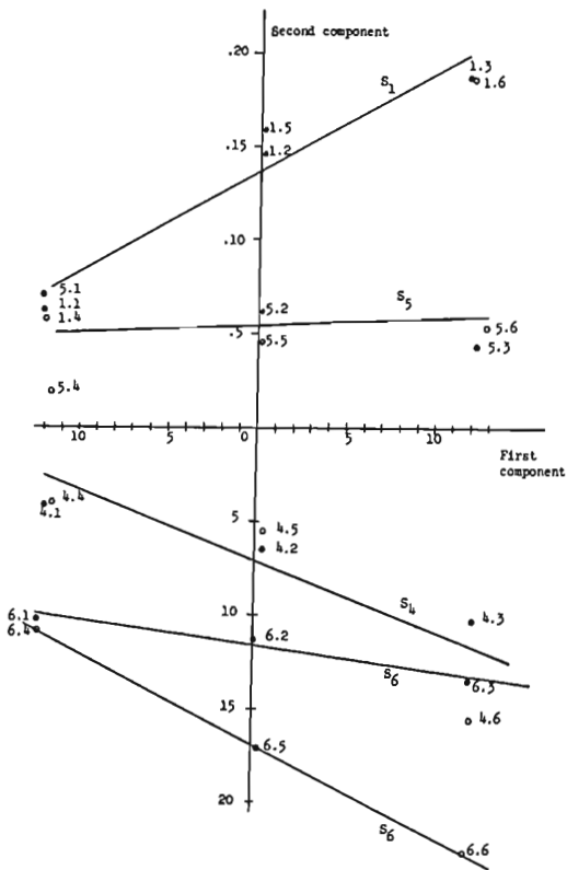
Chart 1. Configuration of the points with respect to the first two Principal Components. The points A.1, A.2, A.3 represent the measurements at three concentrations with spectrophotometer S_4 and the points A.4, A.5, A.6 the corresponding measurements on a subsequent day.
