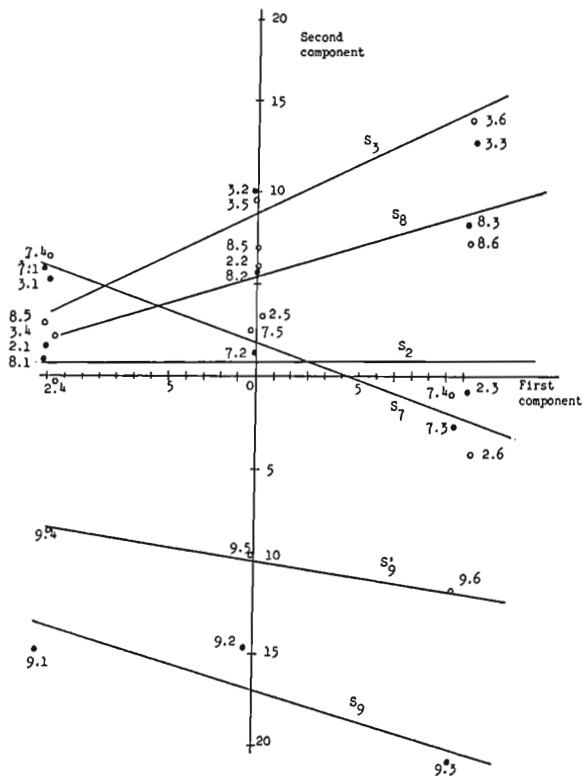
Chart 2. Configuration of the points with respect to the first two Principal Components etc.
