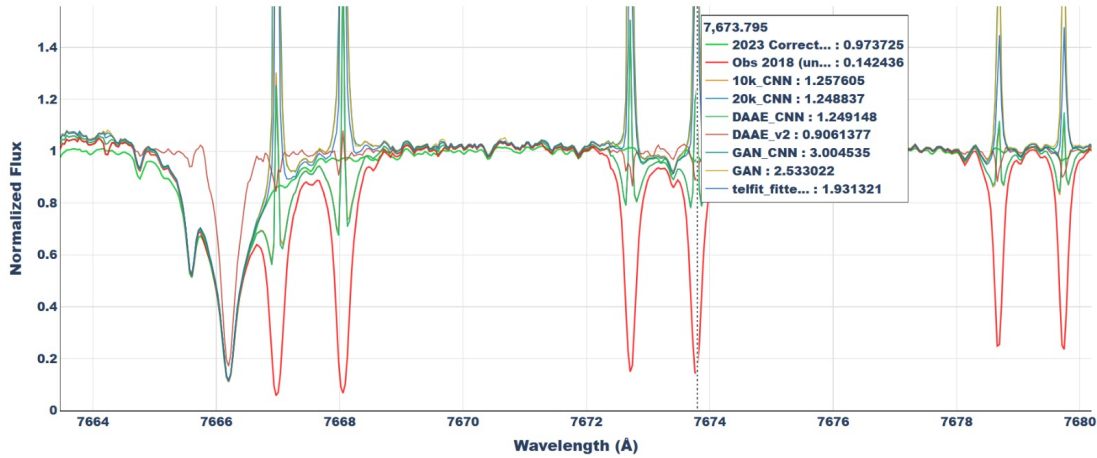
Figure 5.2: Step 4 telluric corrected spectra from all seven model variations are overlaid on the reference spectrum (green) and the telluric contaminated observed spectrum (red). DAAE (deep orange) replicates the reference most closely at deep telluric lines. The Telfit fitted spectrum over-corrects with flux reaching 1.93. The CycleGAN variants (GAN, GAN_CNN) produce spikes with flux exceeding 2.5.
