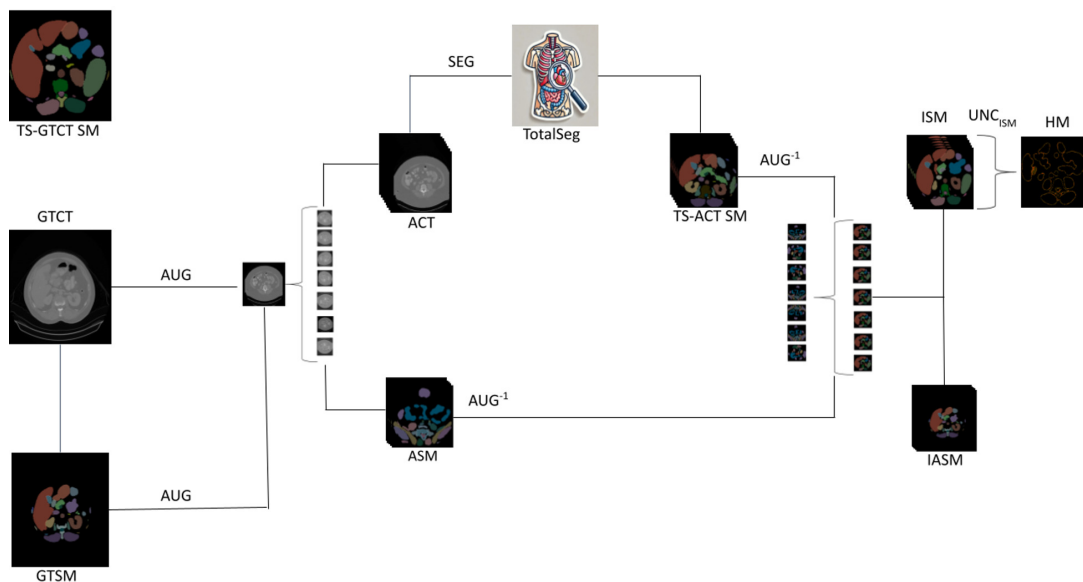
Figure 4.2: Overview of the uncertainty-aware evaluation framework. The original image and its augmented versions are processed by the segmentation model. The augmented predictions are then inverse-transformed back to the original coordinate space to compute the spatial consistency (Dice score) and voxel-wise uncertainty. Reproduced from Sayed et al. [1].
