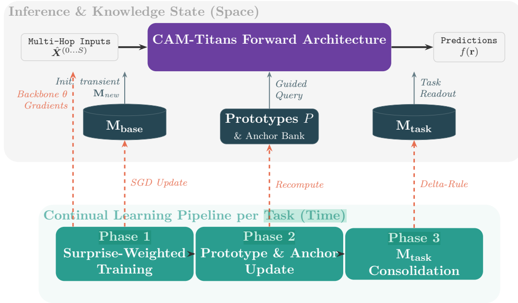
Figure 5.1: Flowchart of the Forward Architecture
