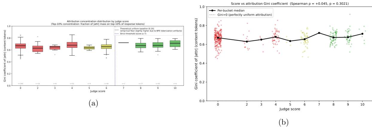
Figure 6.1: Measures of attribution concentration. (a) Distribution of Gini coefficients across score buckets. All buckets sit in the range 0.62–0.72; no monotonic trend is visible. (b) Relationship between attribution concentration and judge score. The Spearman rank correlation is \rho = +0.045 ( p = 0.30 ), not significant. Both analyses indicate little evidence that higher scores are associated with systematically more concentrated token-level attributions.
