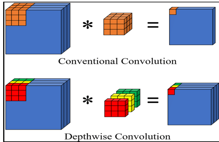
Figure 2.5: Depthwise Convolution
