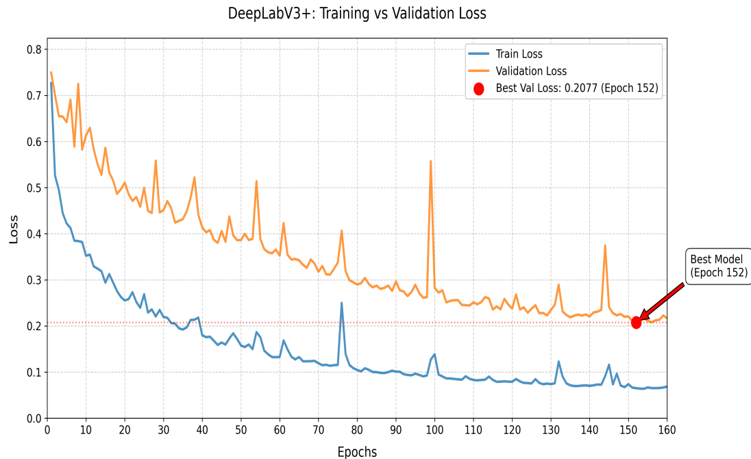
Figure 5.6: Training Vs Validation Loss of DeepLabV3+
