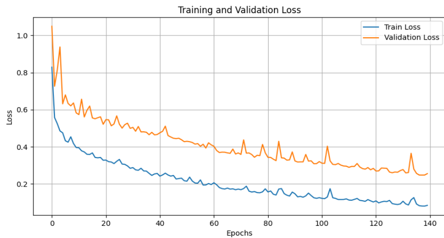
Figure 5.4: Training Vs Validation Loss of Attention Net
