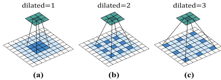
Figure 2.4: Dialated Convolution
