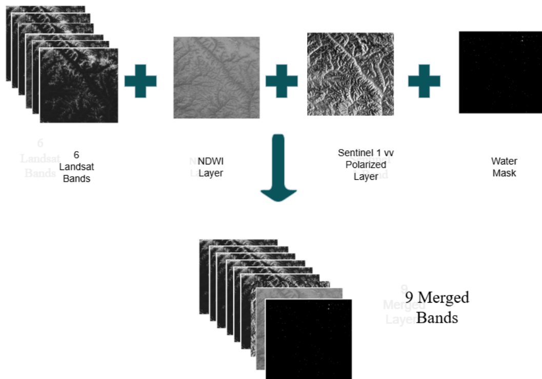
Figure 4.1: Input Structure
