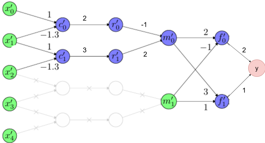
FIGURE 7.3: Abstraction Example
