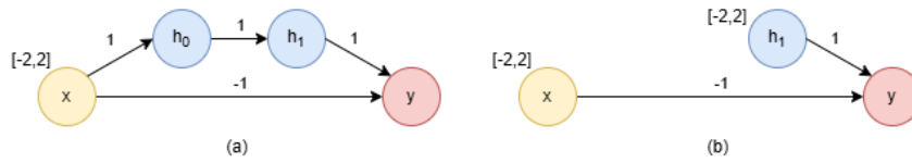
FIGURE 7.1: Illustrative example: (a) Original Network \mathcal{N} , (b) Abstracted Network \mathcal{N}_A with neuron h_0 removed.
