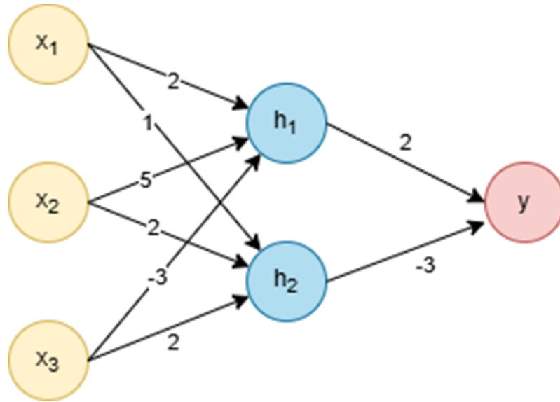
FIGURE 3.3: SDNN example
